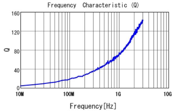
■ LQP03TN0N8B02 Q
