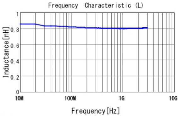
■ LQP03TN0N8B02 L
