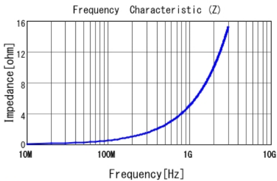
■ LQP03TN0N8B02 |Z|
