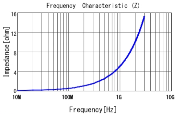
■ LQP03TN0N8C02 |Z|
