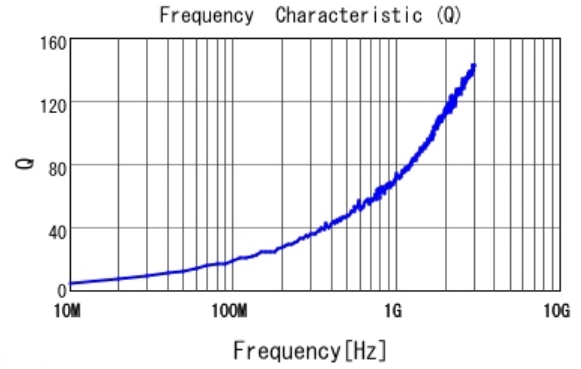
■ LQP03TN0N8C02 Q
