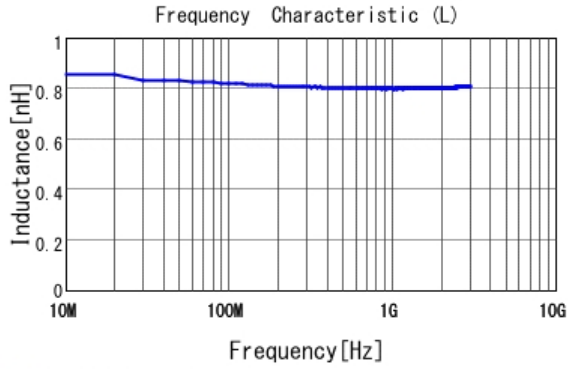
■ LQP03TN0N8C02 L
