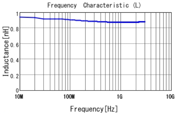
■ LQP03TN0N9B02 L
