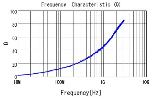
■ LQP03TN0N9B02 Q
