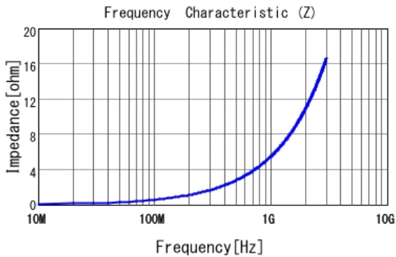
■ LQP03TN0N9B02 |Z|
