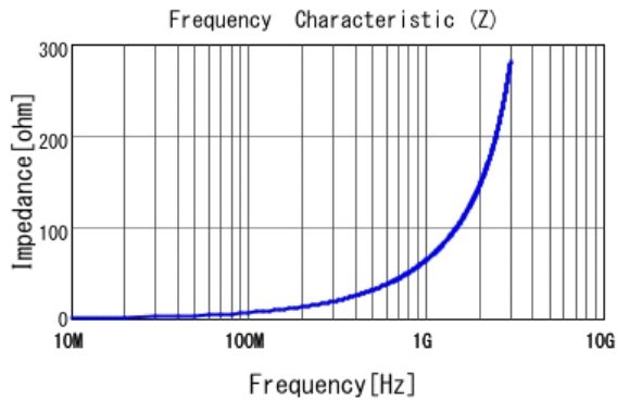
■ LQP03TN10NJ02 |Z|
