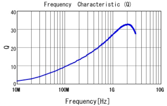
■ LQP03TN10NJ02 Q
