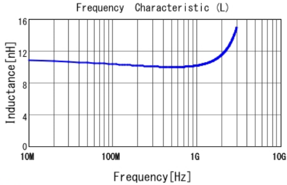
■ LQP03TN10NJ02 L
