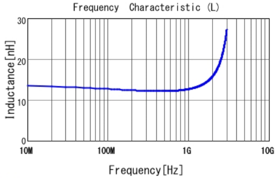
■ LQP03TN12NH02 L
