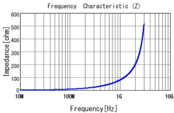
■ LQP03TN12NJ02 |Z|
