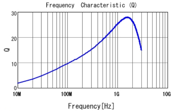
■ LQP03TN12NJ02 Q
