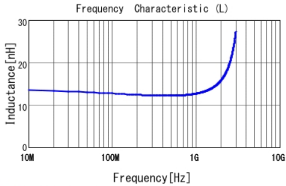
■ LQP03TN12NJ02 L
