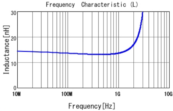
■ LQP03TN13NJ02 L
