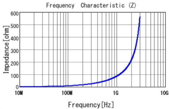
■ LQP03TN13NJ02 |Z|
