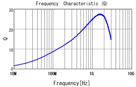
■ LQP03TN13NJ02 Q
