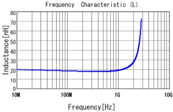
■ LQP03TN18NJ02 L
