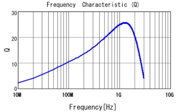
■ LQP03TN18NJ02 Q
