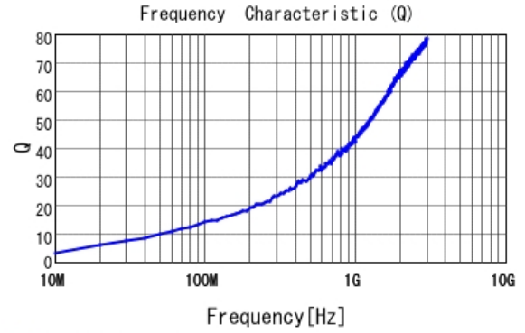
■ LQP03TN1N0B02 Q
