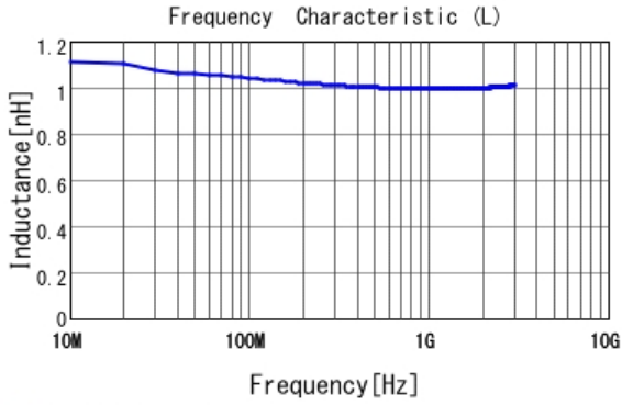
■ LQP03TN1N0B02 L
