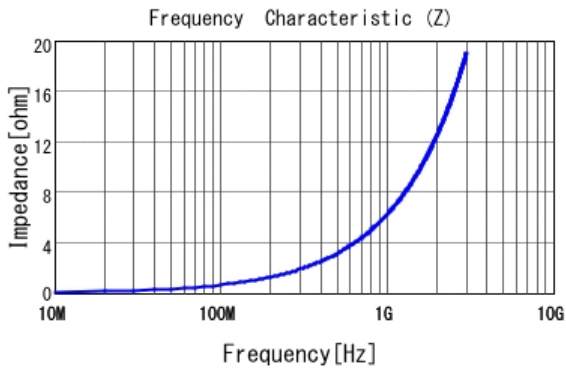
■ LQP03TN1N0B02 |Z|
