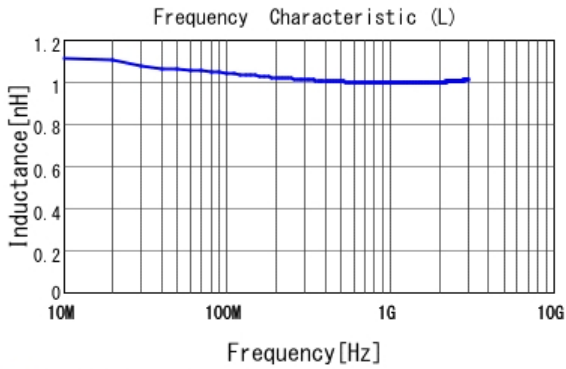
■ LQP03TN1N0C02 L
