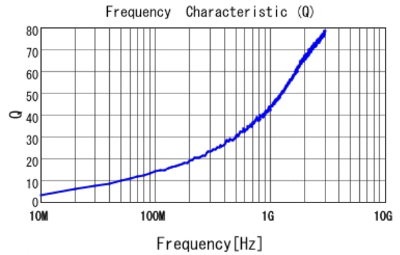
■ LQP03TN1N0C02 Q
