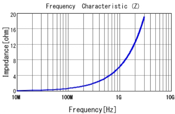
■ LQP03TN1N0C02 |Z|
