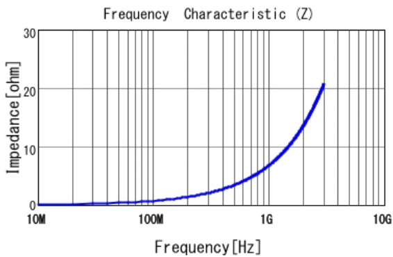
■ LQP03TN1N1C02 |Z|
