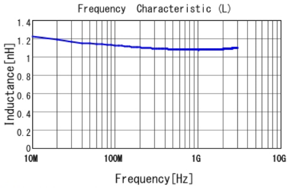
■ LQP03TN1N1C02 L
