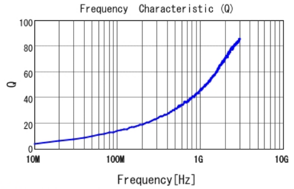
■ LQP03TN1N1C02 Q
