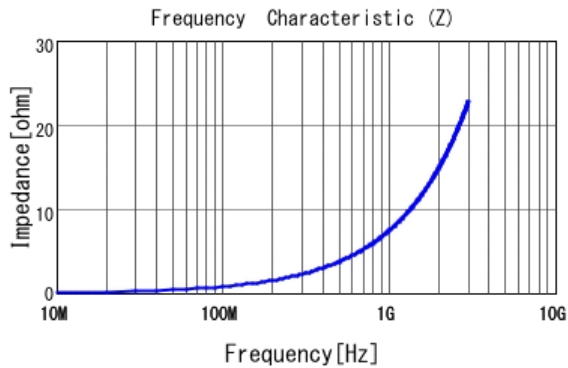
■ LQP03TN1N2B02 |Z|
