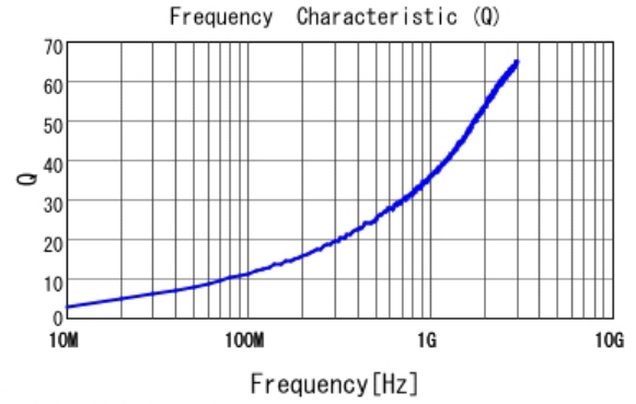
■ LQP03TN1N2B02 Q
