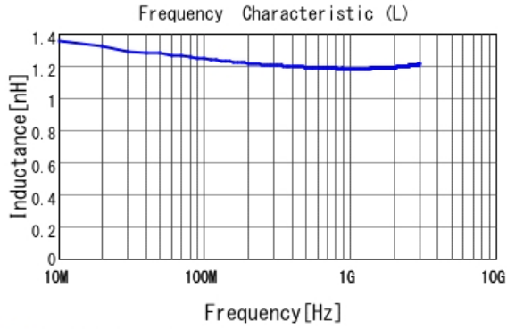
■ LQP03TN1N2B02 L
