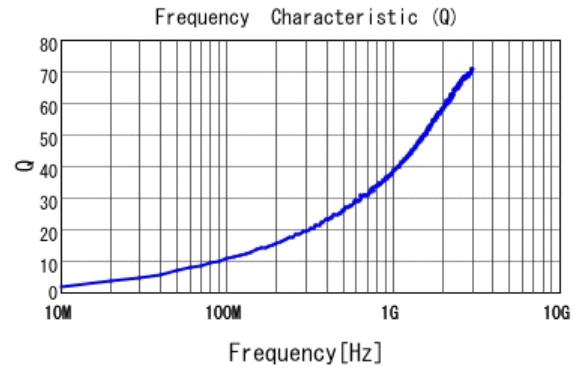
■ LQP03TN1N3B02 Q
