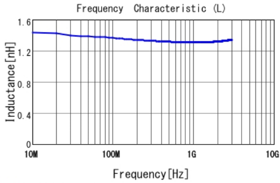
■ LQP03TN1N3B02 L
