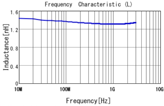
■ LQP03TN1N3C02 L
