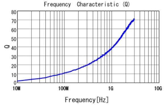
■ LQP03TN1N3C02 Q
