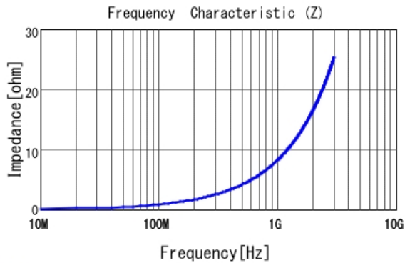
■ LQP03TN1N3C02 |Z|
