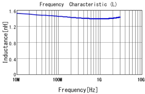
■ LQP03TN1N4B02 L
