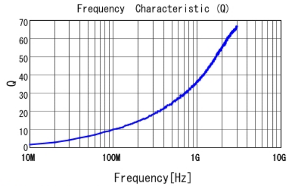
■ LQP03TN1N4B02 Q
