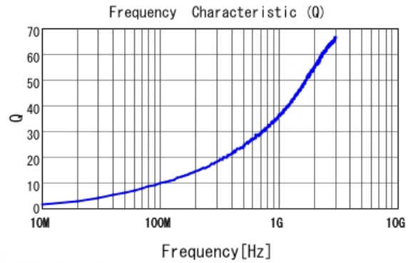
■ LQP03TN1N4BZ2 Q
