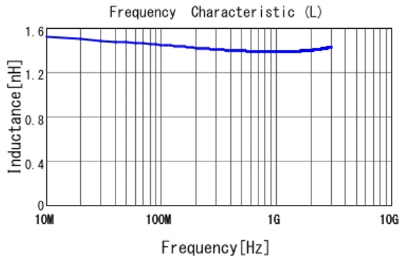
■ LQP03TN1N4BZ2 L
