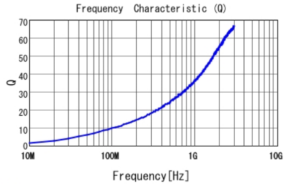
■ LQP03TN1N4C02 Q
