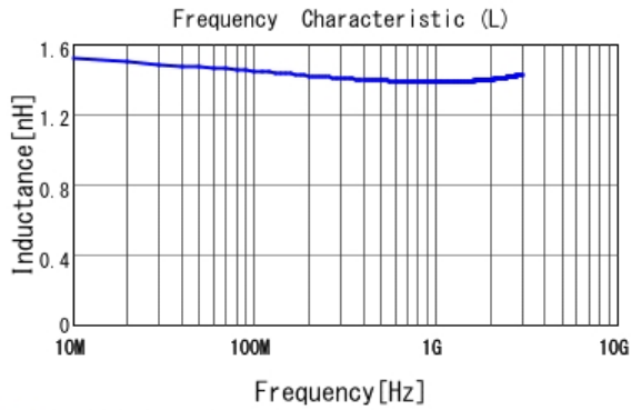
■ LQP03TN1N4C02 L
