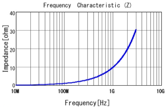
■ LQP03TN1N5B02 |Z|
