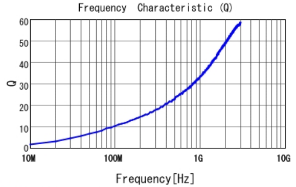
■ LQP03TN1N5B02 Q
