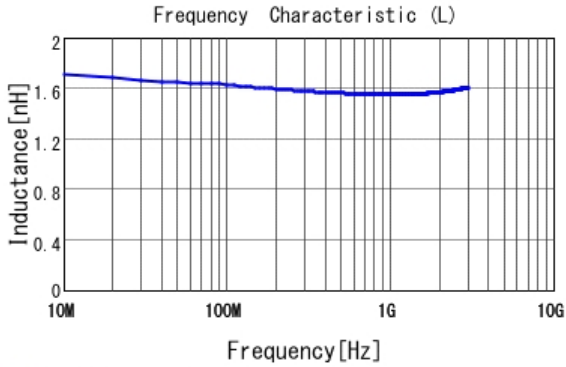
■ LQP03TN1N5B02 L
