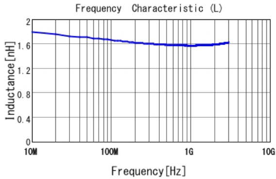
■ LQP03TN1N6B02 L
