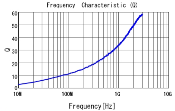
■ LQP03TN1N6B02 Q
