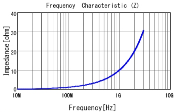
■ LQP03TN1N6B02 |Z|
