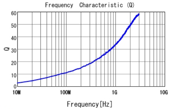
■ LQP03TN1N6C02 Q
