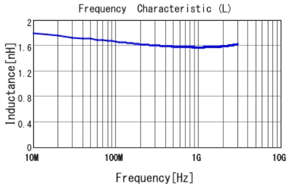
■ LQP03TN1N6C02 L
