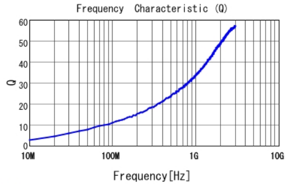
■ LQP03TN1N7C02 Q
