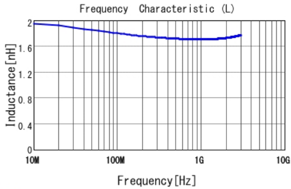
■ LQP03TN1N7C02 L
