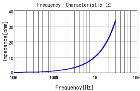
■ LQP03TN1N7C02 |Z|
