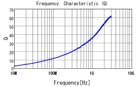
■ LQP03TN1N8B02 Q
