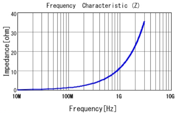
■ LQP03TN1N8B02 |Z|
