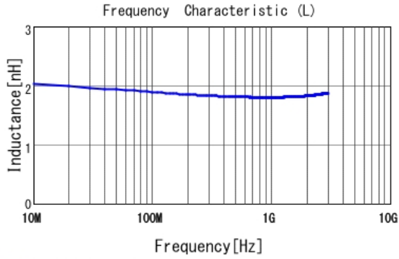
■ LQP03TN1N8B02 L
