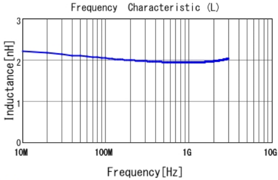
■ LQP03TN1N9B02 L
