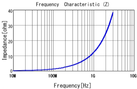
■ LQP03TN1N9B02 |Z|
