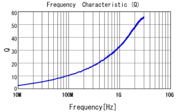
■ LQP03TN1N9B02 Q
