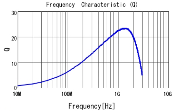
■ LQP03TN20NJ02 Q
