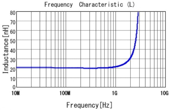
■ LQP03TN20NJ02 L
