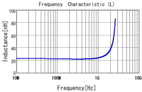
■ LQP03TN22NH02 L
