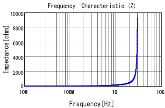
■ LQP03TN22NH02 |Z|
