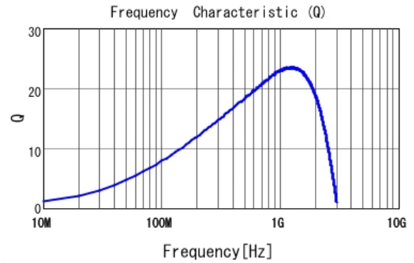
■ LQP03TN22NH02 Q
