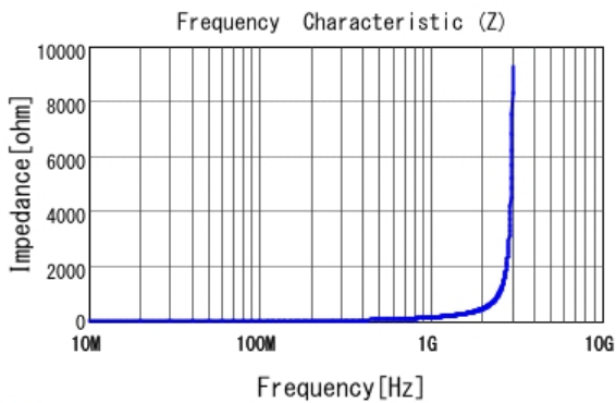
■ LQP03TN22NJ02 |Z|
