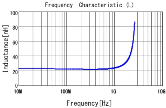
■ LQP03TN22NJ02 L
