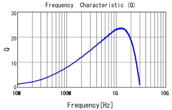
■ LQP03TN22NJ02 Q
