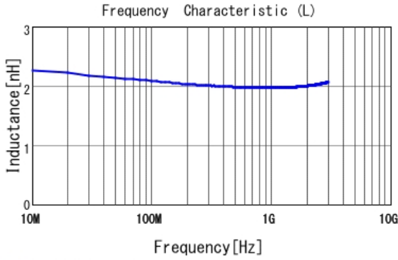
■ LQP03TN2N0B02 L
