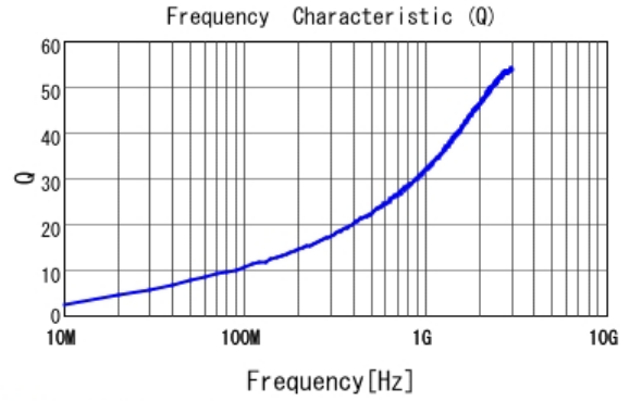
■ LQP03TN2N0B02 Q
