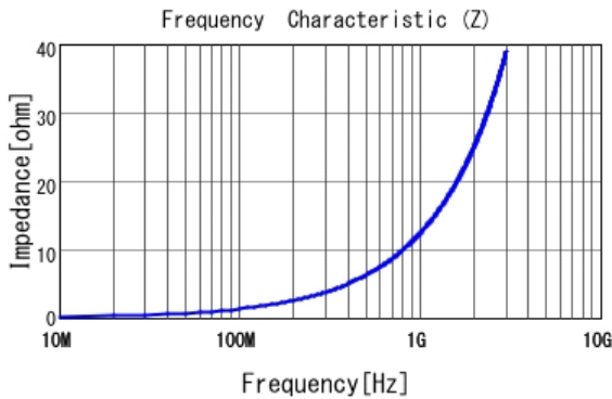
■ LQP03TN2N0B02 |Z|
