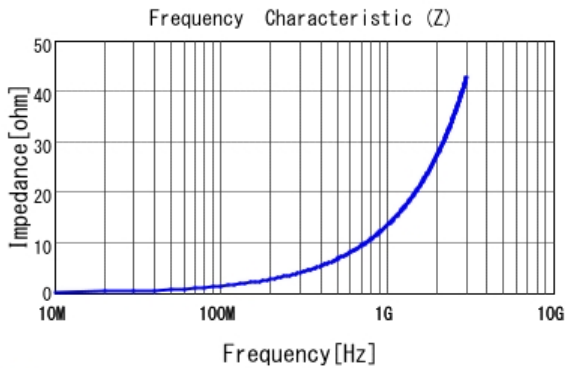
■ LQP03TN2N1BZ2 |Z|
