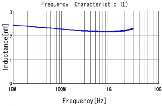
■ LQP03TN2N1BZ2 L
