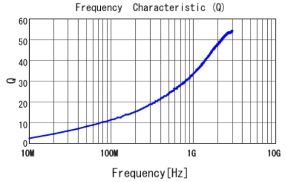
■ LQP03TN2N1BZ2 Q
