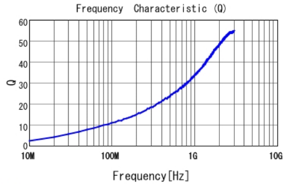
■ LQP03TN2N2B02 Q
