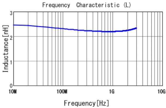
■ LQP03TN2N2B02 L
