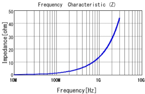
■ LQP03TN2N2B02 |Z|
