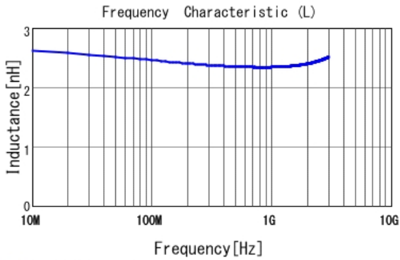
■ LQP03TN2N3B02 L
