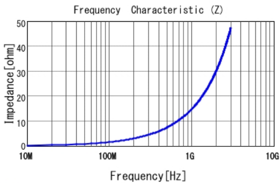
■ LQP03TN2N3B02 |Z|
