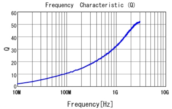
■ LQP03TN2N3B02 Q
