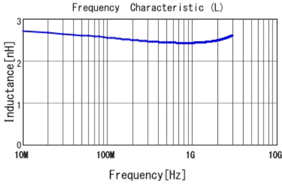
■ LQP03TN2N4B02 L
