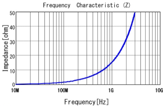
■ LQP03TN2N4B02 |Z|
