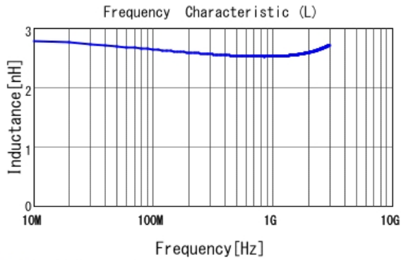
■ LQP03TN2N5C02 L
