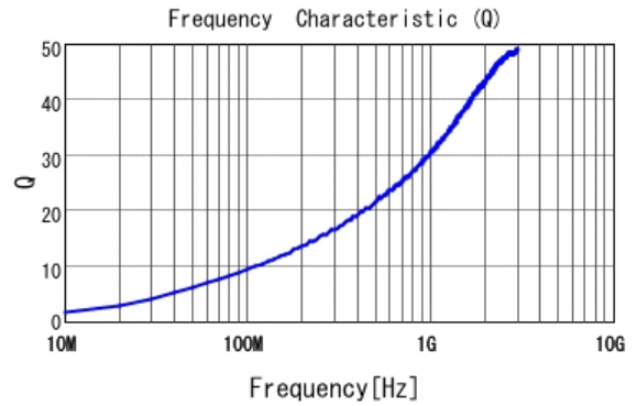
■ LQP03TN2N5C02 Q
