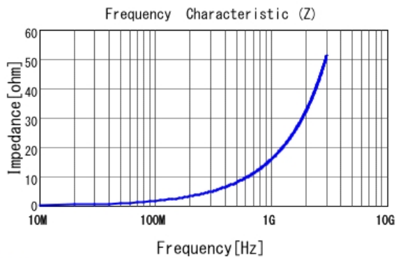
■ LQP03TN2N5C02 |Z|
