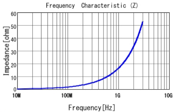
■ LQP03TN2N6B02 |Z|
