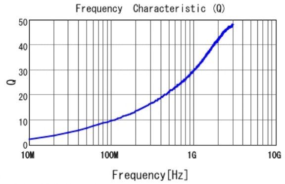
■ LQP03TN2N6B02 Q
