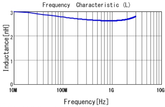
■ LQP03TN2N6B02 L
