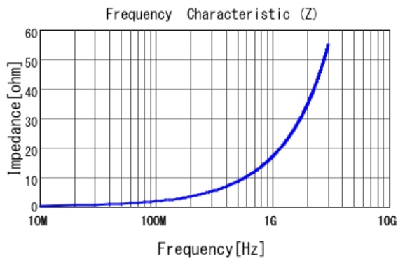
■ LQP03TN2N7B02 |Z|
