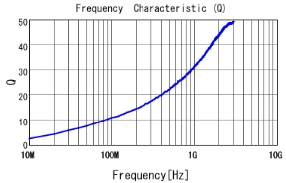
■ LQP03TN2N7B02 Q
