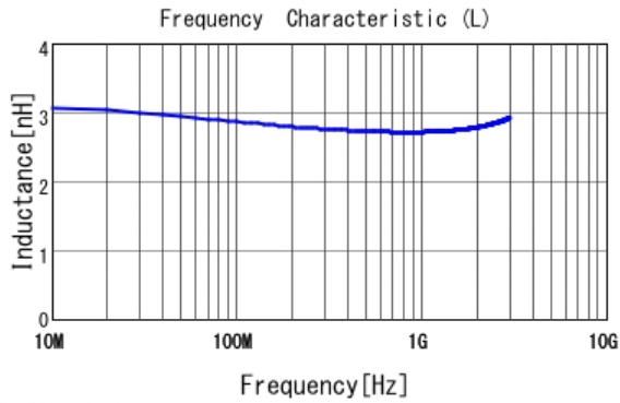
■ LQP03TN2N7B02 L
