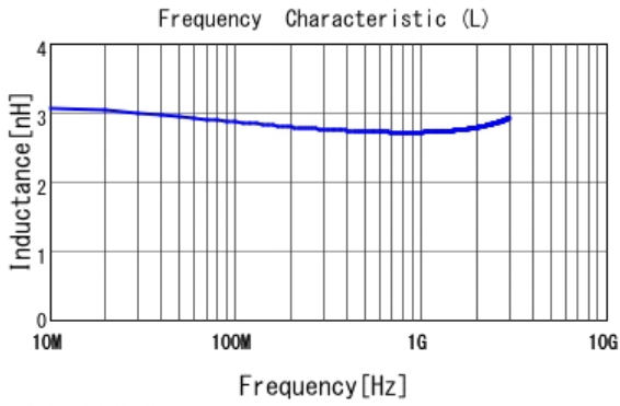
■ LQP03TN2N7C02 L
