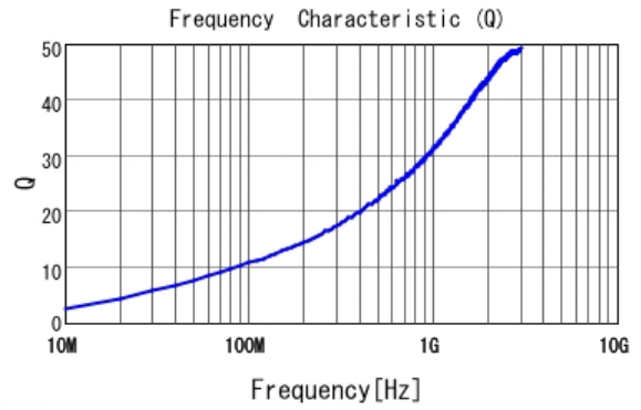
■ LQP03TN2N7C02 Q
