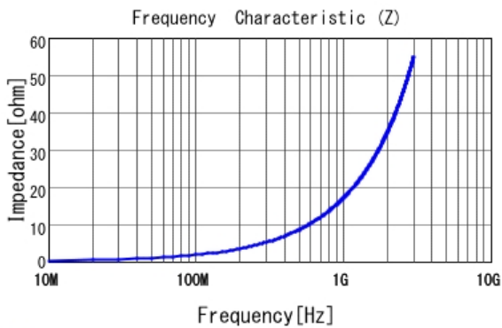
■ LQP03TN2N7C02 |Z|
