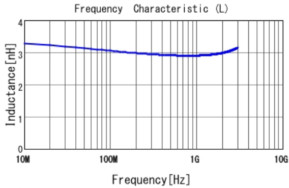
■ LQP03TN2N9B02 L
