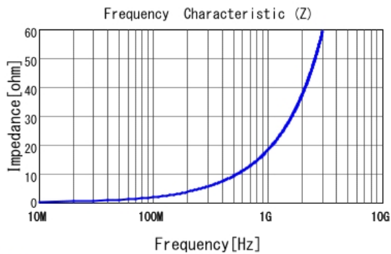
■ LQP03TN2N9B02 |Z|
