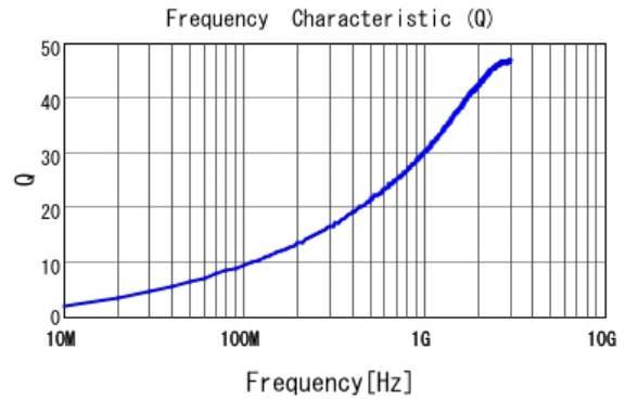
■ LQP03TN2N9B02 Q
