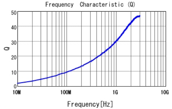
■ LQP03TN2N9C02 Q
