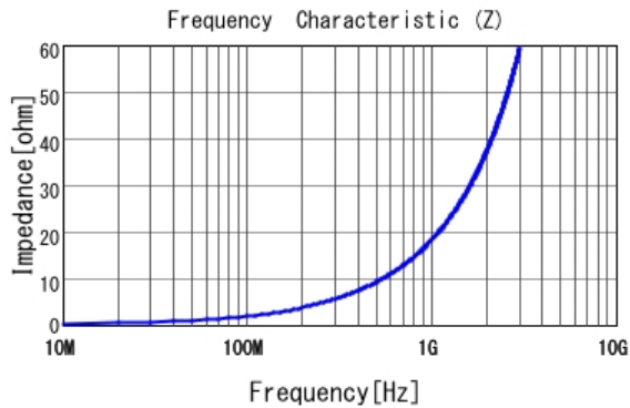
■ LQP03TN2N9C02 |Z|
