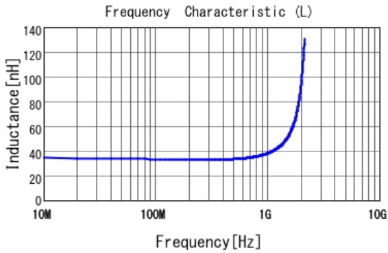
■ LQP03TN33NJ02 L
