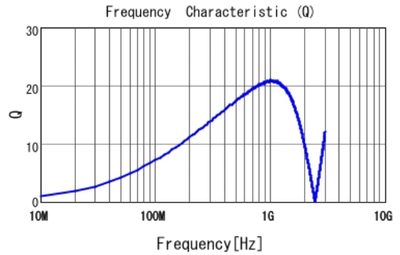
■ LQP03TN33NJ02 Q
