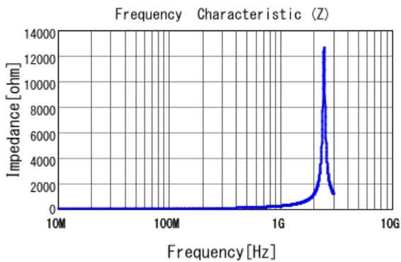
■ LQP03TN33NJ02 |Z|
