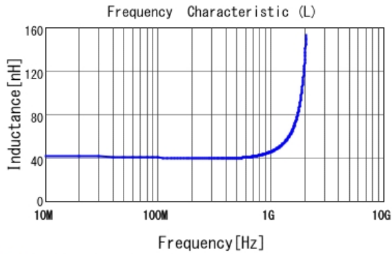
■ LQP03TN39NJ02 L
