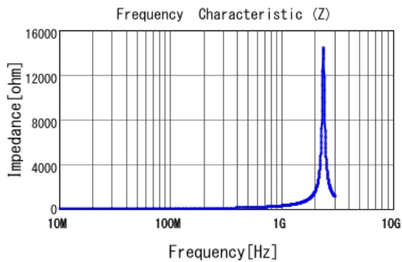
■ LQP03TN39NJ02 |Z|
