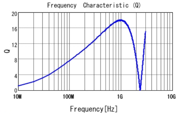
■ LQP03TN39NJ02 Q
