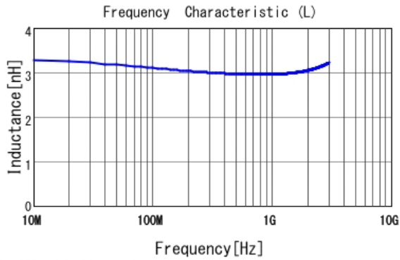
■ LQP03TN3N0B02 L
