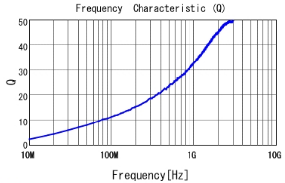
■ LQP03TN3N0B02 Q
