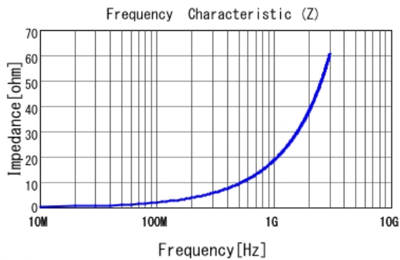
■ LQP03TN3N0B02 |Z|
