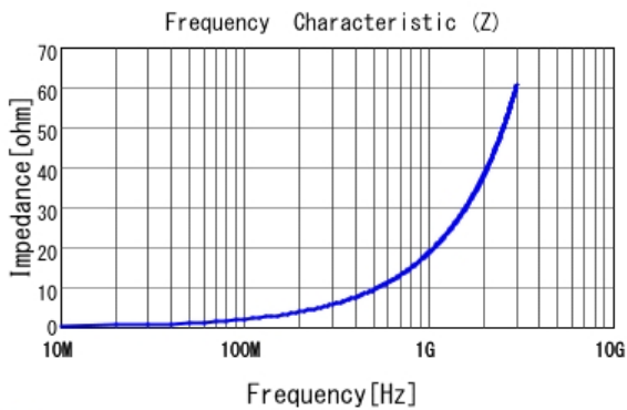
■ LQP03TN3N0C02 |Z|
