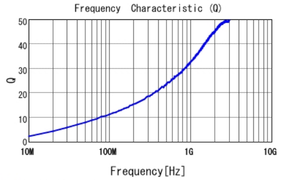
■ LQP03TN3N0C02 Q
