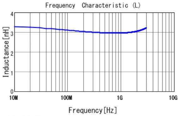
■ LQP03TN3N0C02 L
