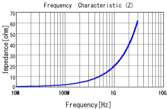
■ LQP03TN3N1B02 |Z|
