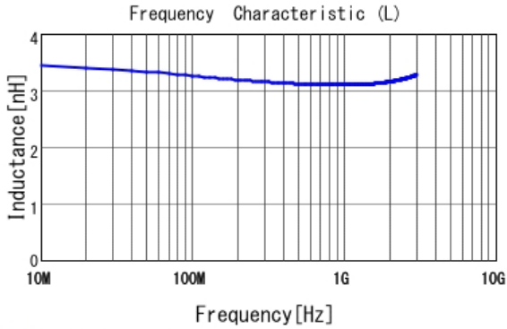
■ LQP03TN3N1B02 L
