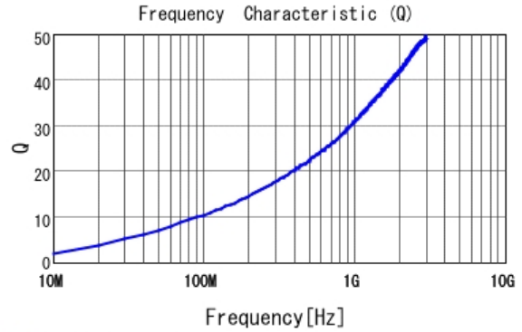
■ LQP03TN3N1B02 Q
