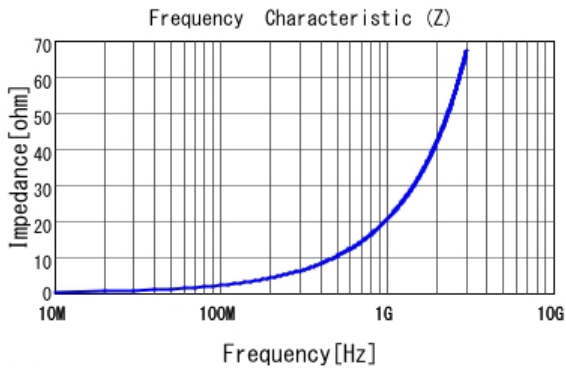
■ LQP03TN3N3B02 |Z|
