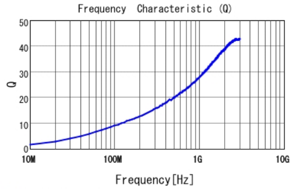
■ LQP03TN3N3B02 Q
