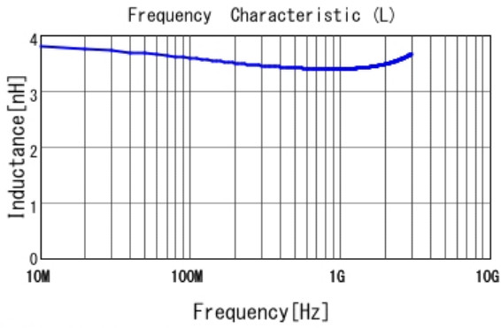
■ LQP03TN3N4C02 L
