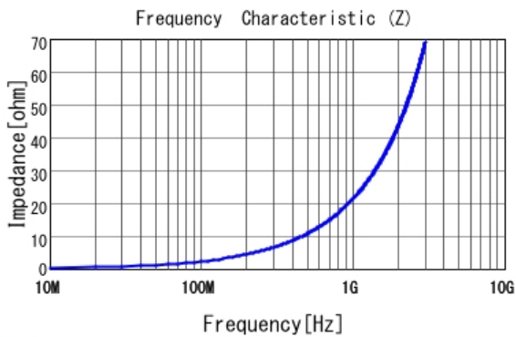
■ LQP03TN3N4C02 |Z|
