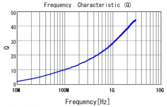
■ LQP03TN3N4C02 Q
