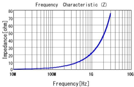
■ LQP03TN3N5C02 |Z|
