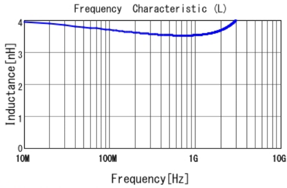
■ LQP03TN3N5C02 L
