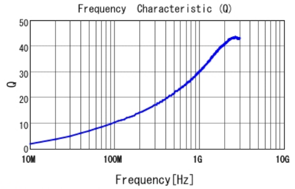
■ LQP03TN3N5C02 Q
