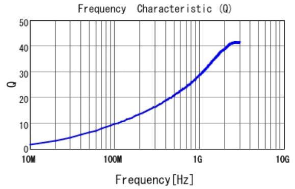
■ LQP03TN3N6B02 Q
