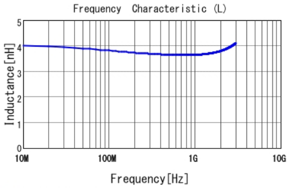
■ LQP03TN3N6B02 L
