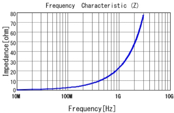
■ LQP03TN3N6C02 |Z|
