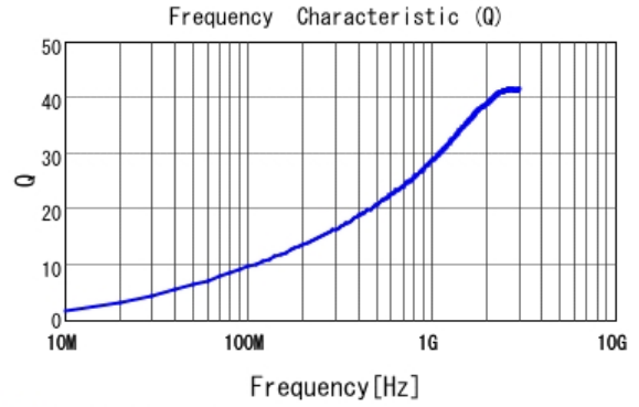
■ LQP03TN3N6C02 Q
