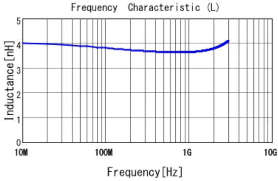
■ LQP03TN3N6C02 L
