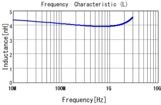
■ LQP03TN3N9B02 L
