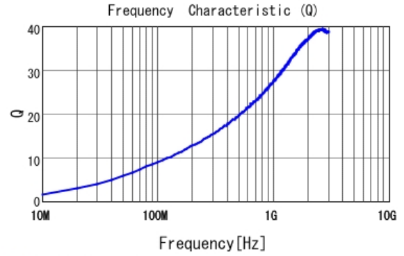
■ LQP03TN3N9B02 Q
