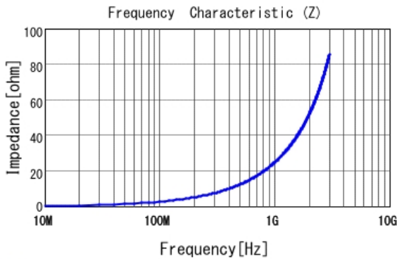
■ LQP03TN3N9B02 |Z|
