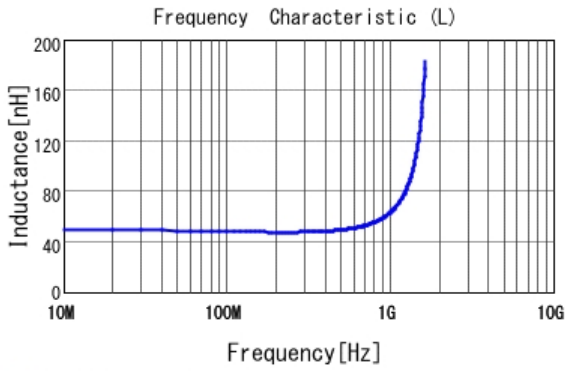
■ LQP03TN47NH02 L
