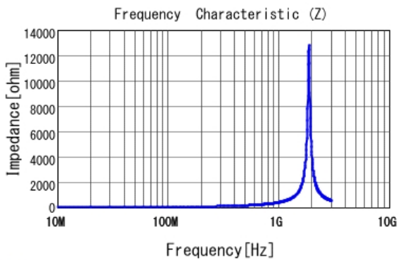
■ LQP03TN47NJ02 |Z|
