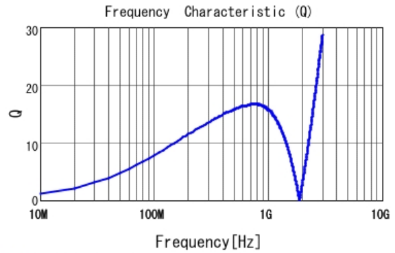
■ LQP03TN47NJ02 Q
