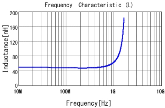
■ LQP03TN47NJ02 L
